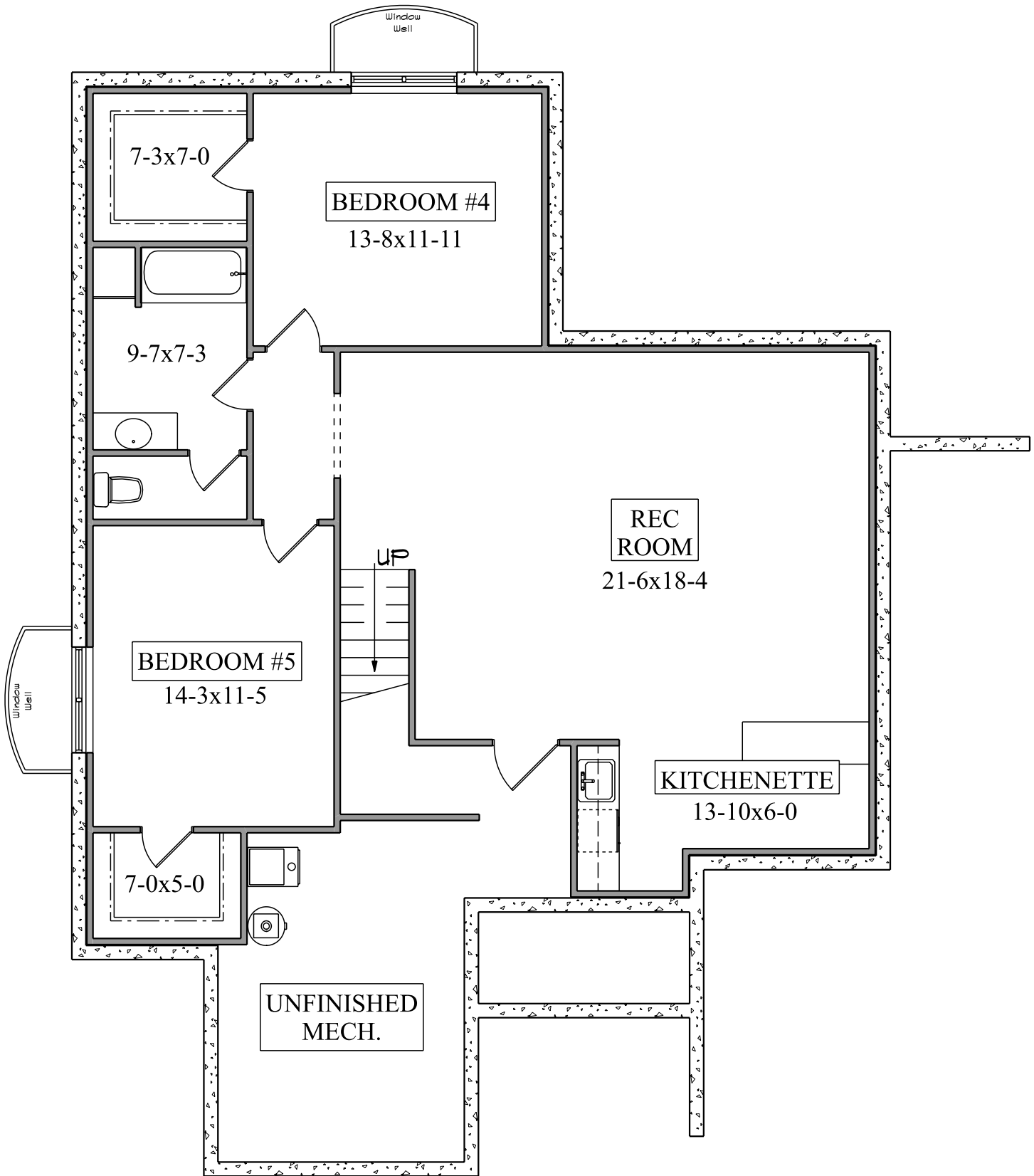
LOWER FLOOR PLAN 1,213 FinSqFt
